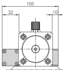
Control valve ONLY in piston rod return
